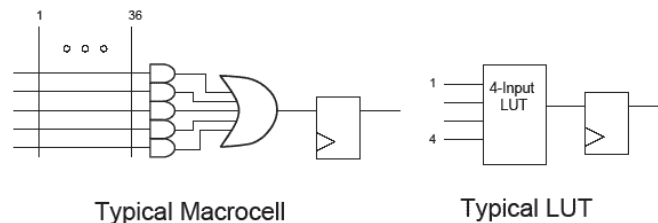
Figure 1 – CPLD Macrocell and FPGA LUT Elements
