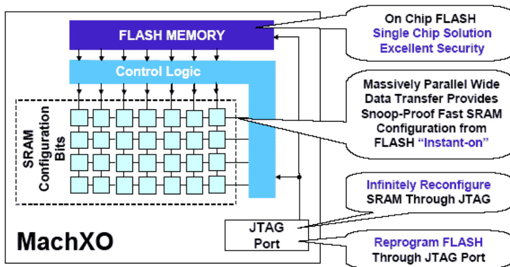
Figure 4 -- MachXO Configuration Memories
