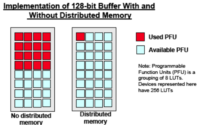
Figure 3 -- Distributed Memory Allows 16X Efficiency Improvement In Buffer Implementation
