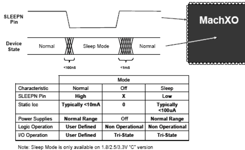
Figure 6 -- MachXO Sleep Mode
